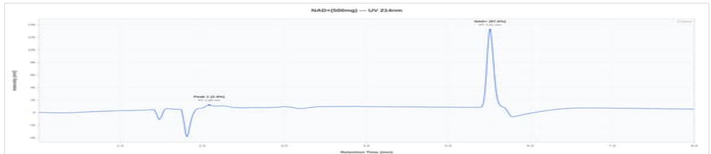
NAD+ 500mg - PP-B1-NAD500: UV Chromatogram
